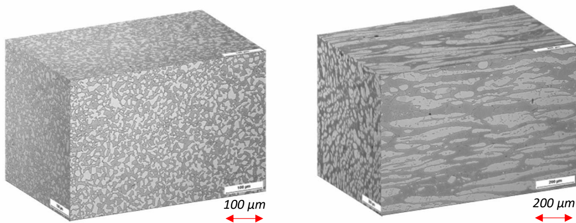
Fine isotropic microstructure of HIPed material vs. forged bar. Note scale marker bar.
